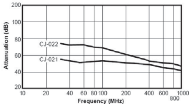
Figure 2 Shielding Effectiveness with 360° Ground Termination
