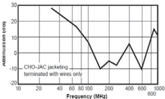
Figure 1 Shielding Effectiveness with Wire Ground Termination
