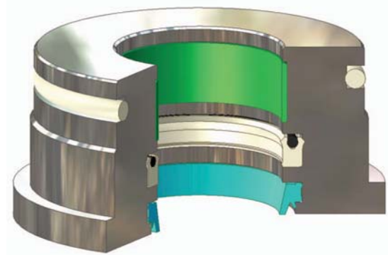
568 installed in Static Head Gland
