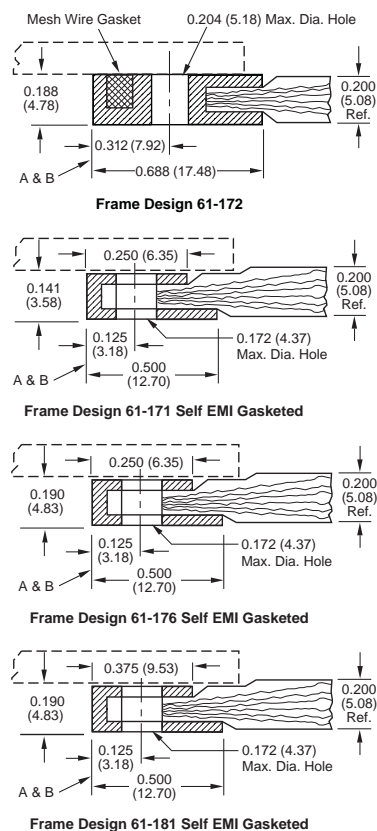
Figure 1 VIP Standard Frame designs (mm dimensions in parentheses)
